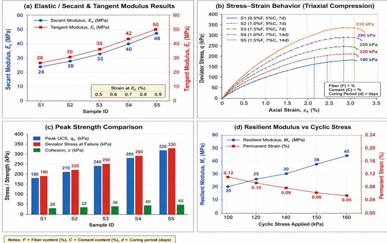
Fig. 16 Simulink results of stress-strain and elastic properties
