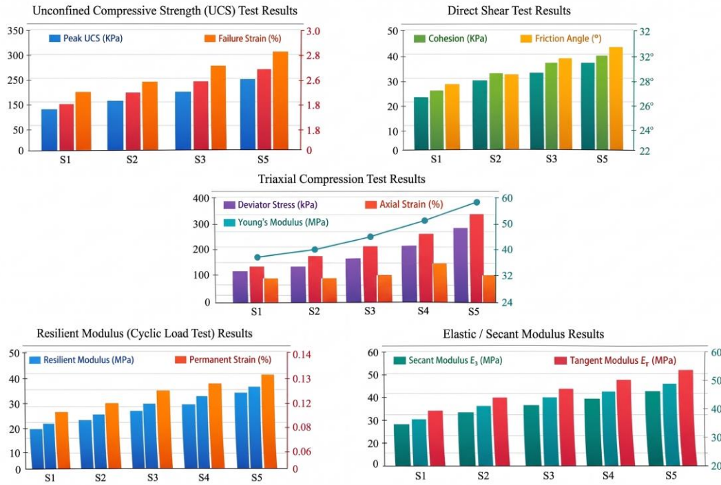
Fig. 13 Comprehensive set of the mechanical and geotechnical properties of fiber-reinforced cement-stabilized Laterite soil samples
