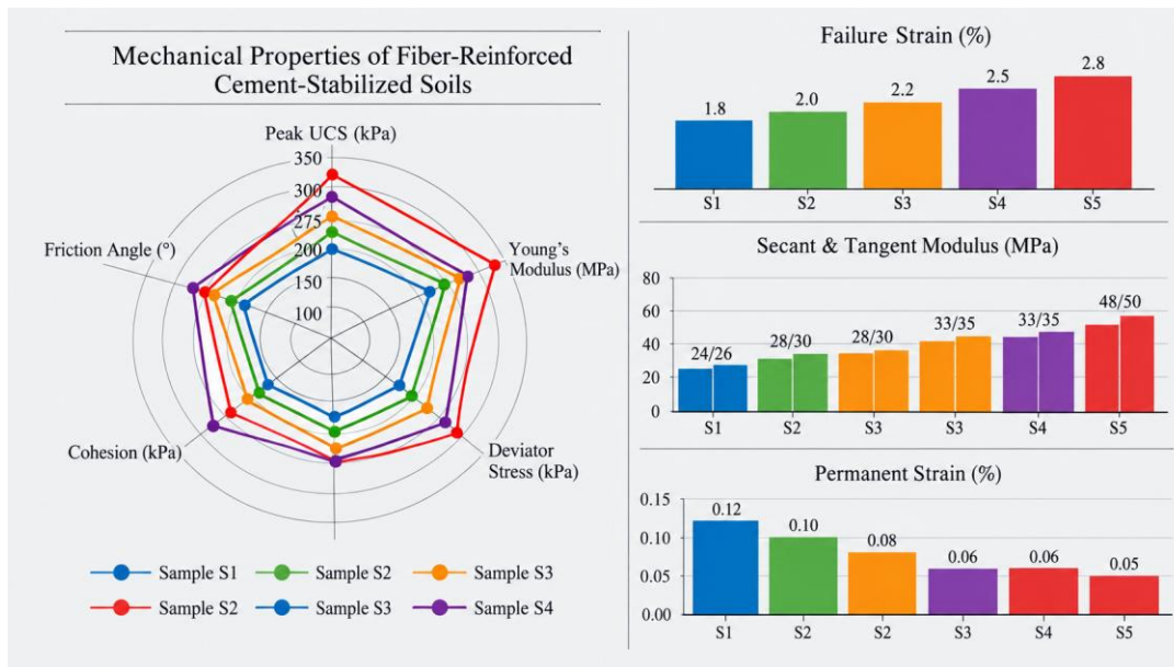
Fig. 14 Visual summary of the mechanical performance of fiber-reinforced cement-stabilized Laterite soils across five samples (S1-S5)
