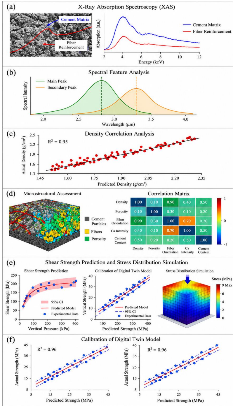
Fig. 7 Integrated X-ray Absorption Spectroscopy (XAS) for proposed technique
