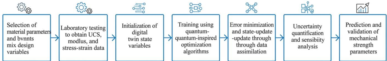
Fig. 1 Process steps for mechanical strength prediction
