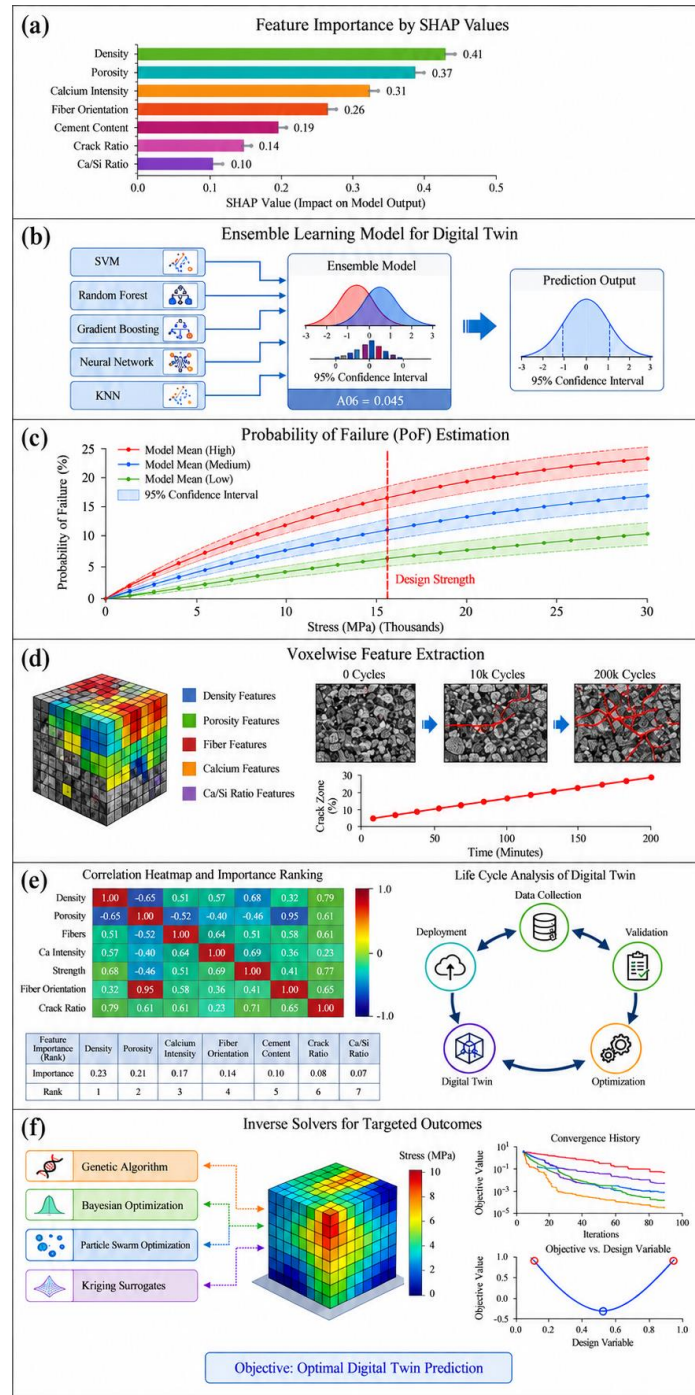
Fig. 11 SHAP values quantify for proposed technique
