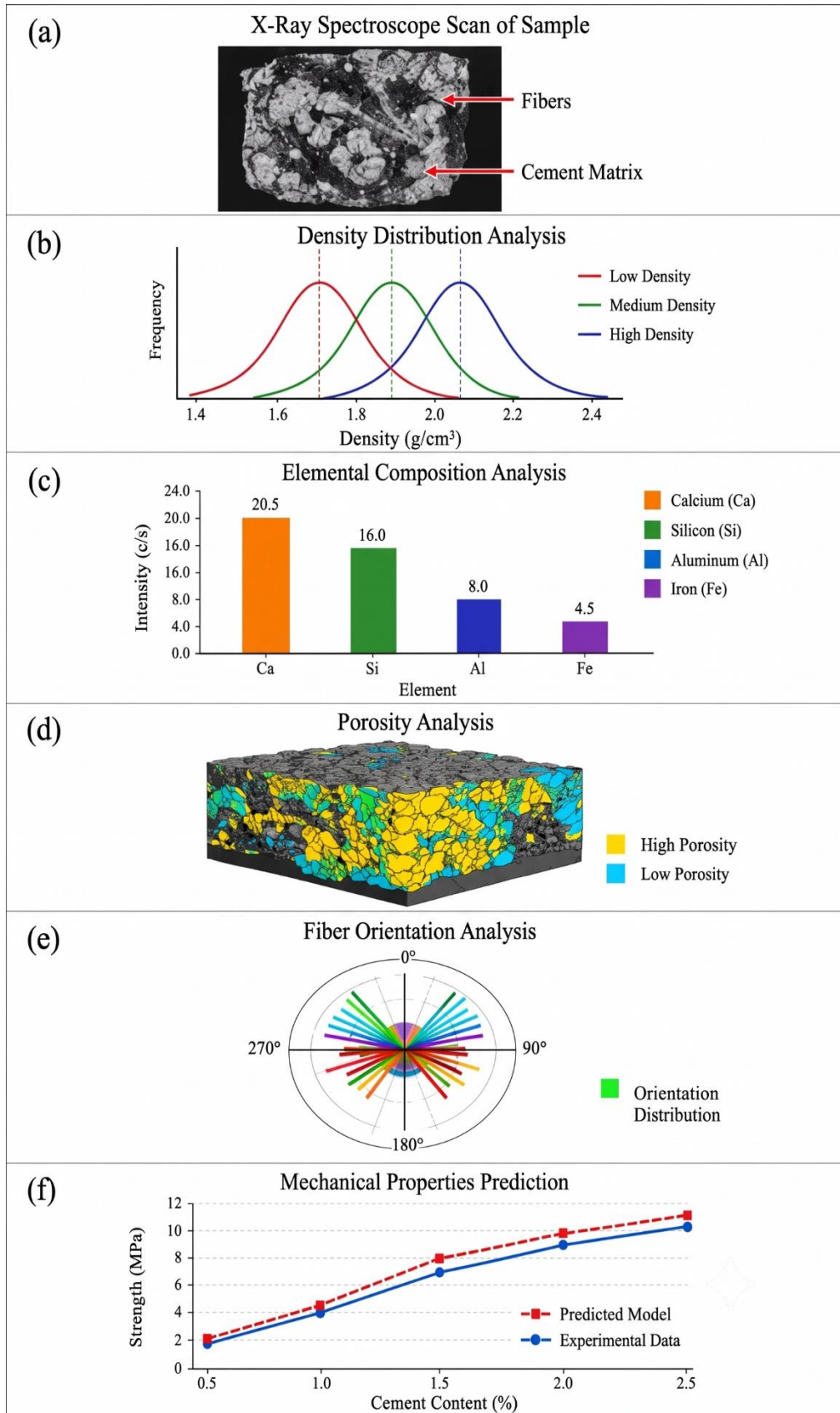
Fig. 6 Multi-scale analysis of Fiber-Reinforced Cement-Stabilized Laterite Soil using proposed technique
