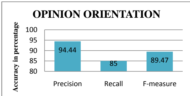
Figure 3. Opinion Orientation
