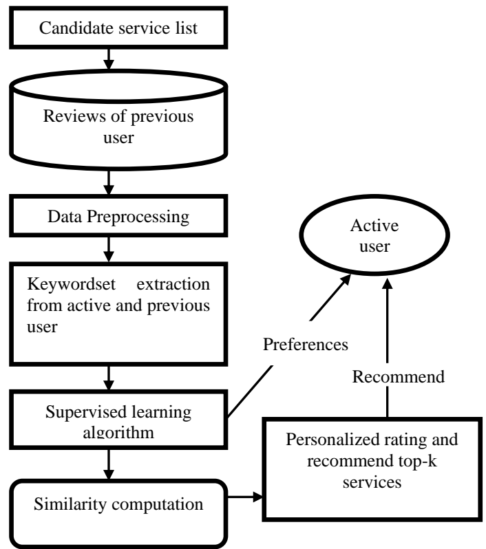
Figure 1. Architectural Diagram
