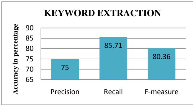
Figure 2. Keyword Extraction
