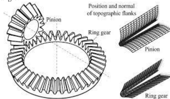
Straight Bevel Gears
