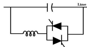
Fig. 8 TCSC structure
