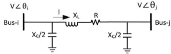
Fig.1 π-model single line diagram
