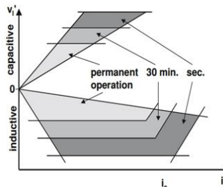
Fig. 9 TCSC operational diagram
