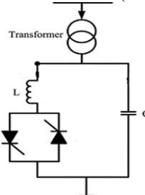
Fig. 4 SVC building block
