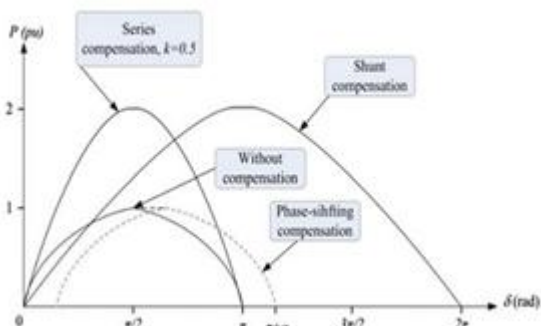
Fig. 3 P-δ curve
