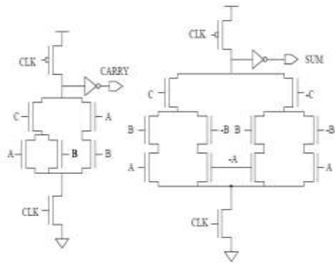
Fig.5.Dual rail domino full adder
