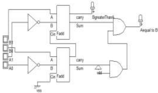
Fig. b. proposed 2-bit comparator
