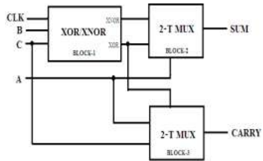
Fig.7. Design technique of Full Adder
