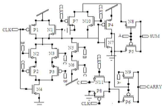
Fig.8. Proposed 1-Bit Domino Full Adder.
