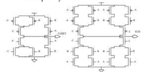
Fig.1. The Schematic Diagram of a 1-bit Static CMOS full adder cell
