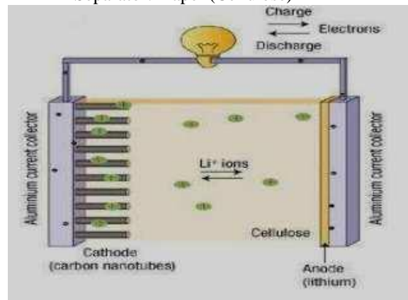
Fig7. Schematic of a Paper Battery
