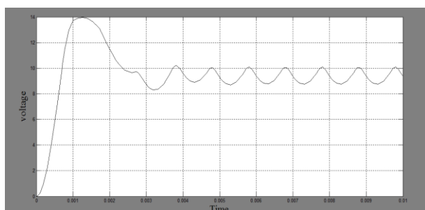
Figure :3 buck converter
