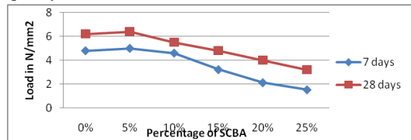
Figure 9.2: line diagram shows the split tensile strength
