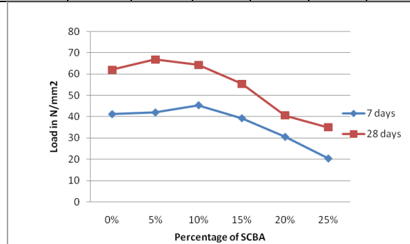
Figure 9.1: line diagram shows the compressive strength
