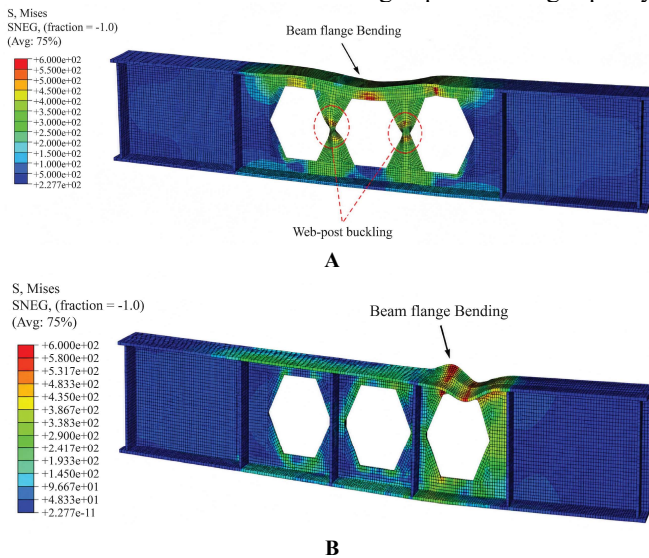
Fig. 10 Failure Modes [50]
