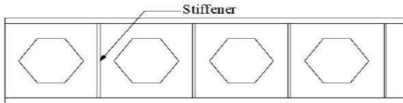
Fig. 9 Hexagonal Castellated Beam with Transverse Stiffeners [30].
