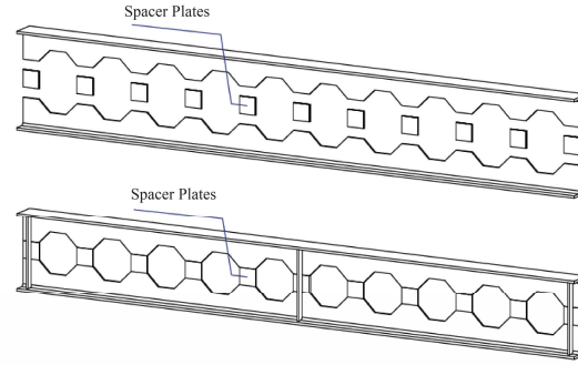
Fig. 15 A Castellated Steel Beam That Has Been Rejoined With an Increment Plate (Octagonal Opening) [61]
