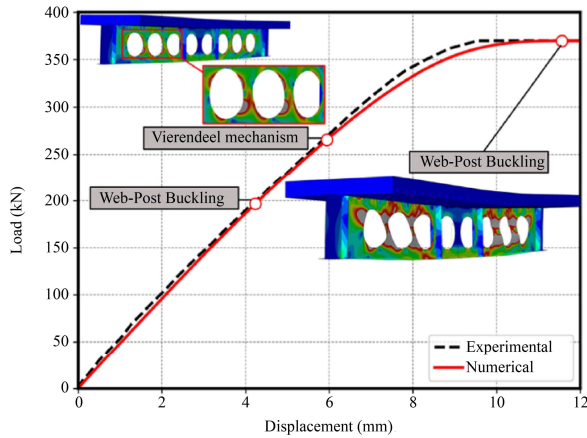
Fig. 17 Load-Displacement Curves: Evaluation of Instability and Behavior [75]
