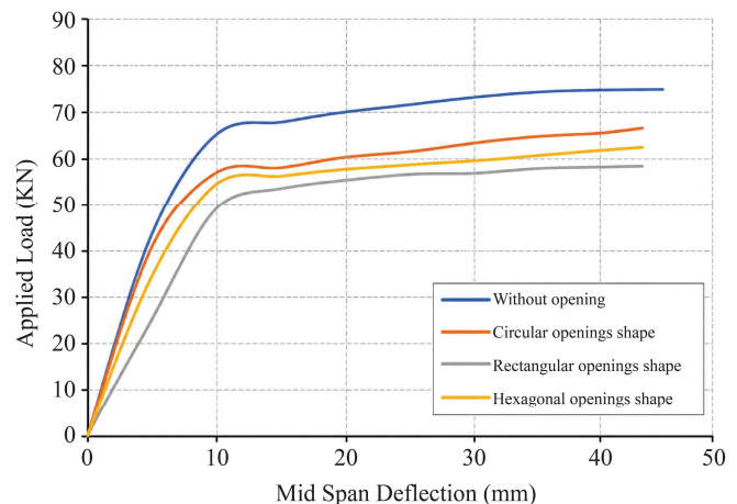
Fig. 4 The Load Against Mid-Span Deflection for Steel Beams with Various Opening Shapes and an Aspect Ratio of 1.71 [22]
