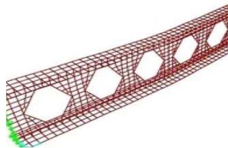
Fig. 7 LTB Deformation and a Typical Finite Element Mesh in FEA [42]
