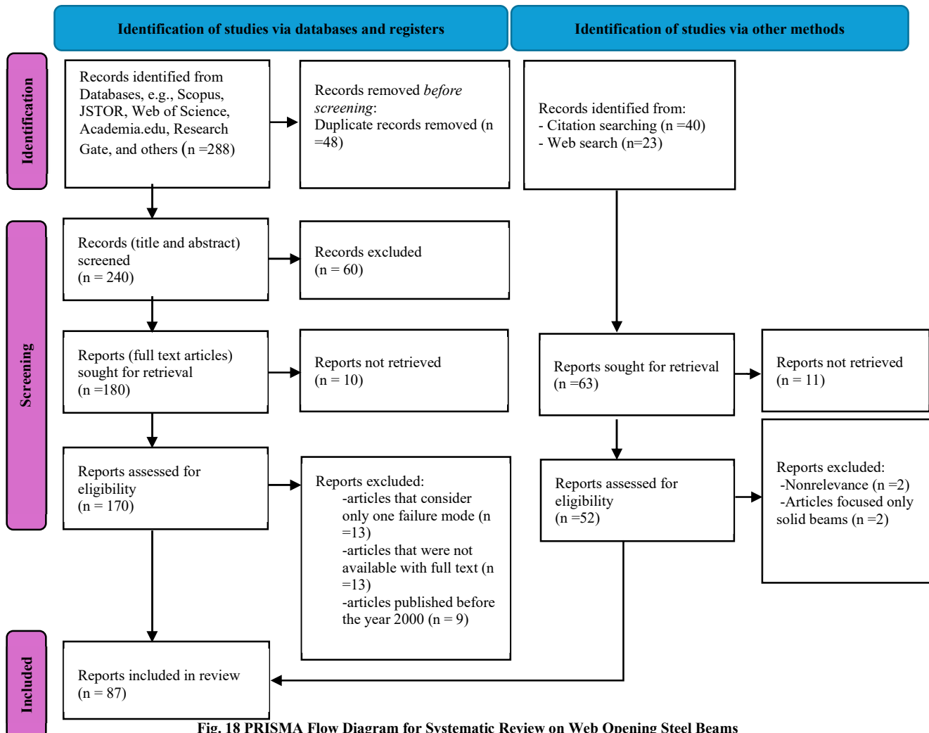
Fig. 18 PRISMA Flow Diagram for Systematic Review on Web Opening Steel Beams
