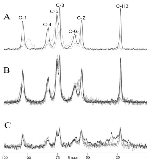
Fig 5: Overlaid CP-MAS Spectra of Standards (A), Extracted Samples (B), and Raw Samples (C)
