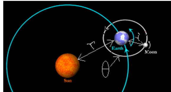
Figure V. Orbit Diagram of the Sun-Earth-Moon System
