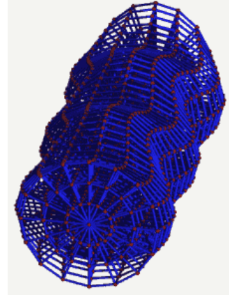
Figure III. Graphical Representation of the Structure of Gravitational Wave (Courtesy: Max Planck Institute of Gravitational Physics)
