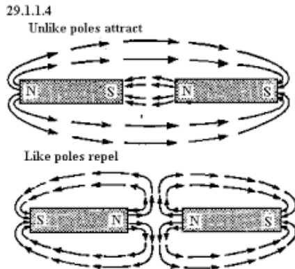
Figure II. Magnetic Forces between Two Pairs of magnets (Courtesy: University of Queensland, Australia)
