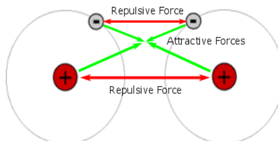
Figure I. Electrostatic Force between two atoms (Courtesy: Quora)
