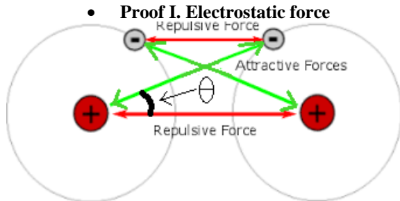
Figure IV. Electrostatic Force Between Two Atoms
