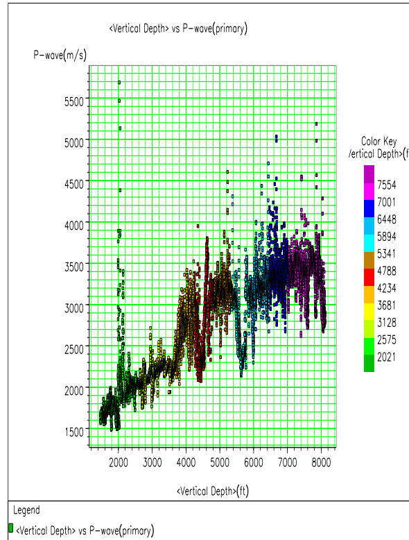
Figure 2: Velocity vs Depth plot for well 01. Velocity increased with depth in the normal trend.
