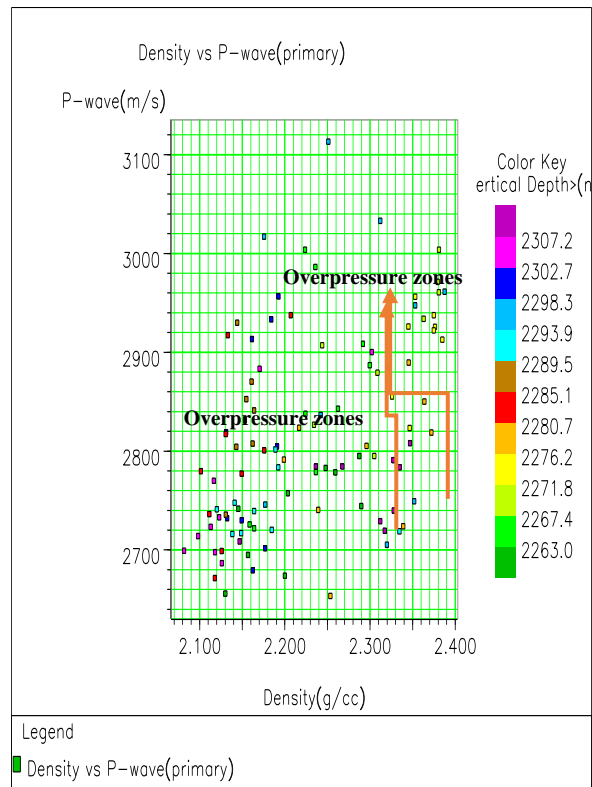
Figure 11: Velocity vs Density cross-plot for well 02. Unloading mechanism is observed from 2289.5m to 2298.3m (blue colour key), while overpressure zones occurred from 2280.7m to 2285.1m (red colour key).
