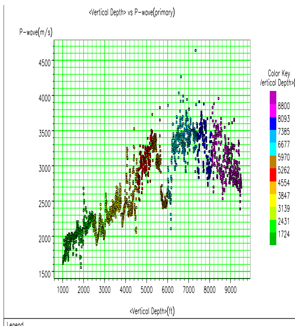
Figure 5: Velocity-Depth plot for well 04. Velocity increased and dropped.
