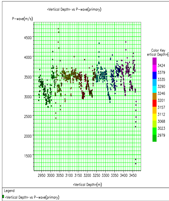
Figure 4: Velocity-Depth plot for well 03. Velocity increased slightly with and remained steady with depth.
