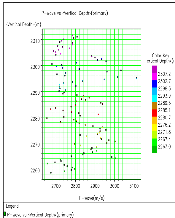
Figure 3: Velocity-Depth plot for well 02. Velocity increased but the trend is not linear.
