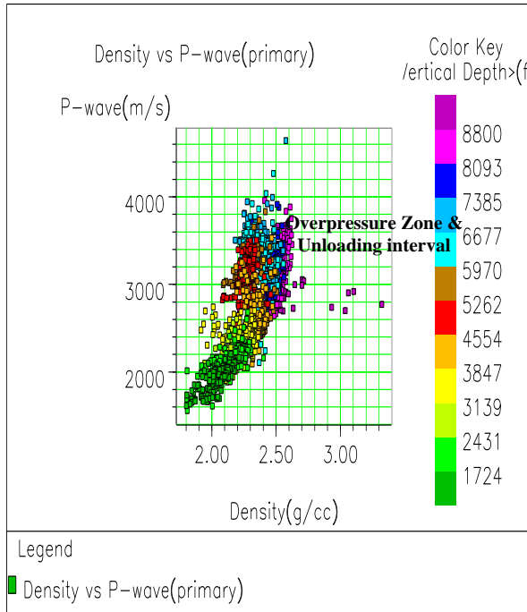
Figure 13: Velocity vs Density cross-plot for well 04. Unloading mechanism is observed from 5970ft to 6677ft (about 215.49m thick), while overpressure zones is observed from 4554ft to 5262ft (about 215.79m thick).
