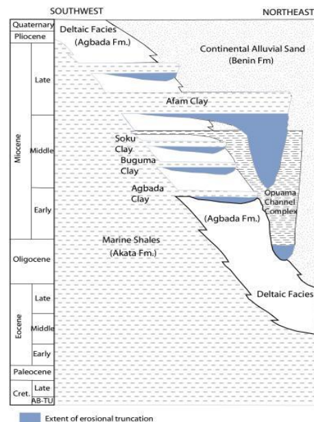
Figure 1: Stratigraphic column of the Niger Delta (Modified from Doust and Omatsola, 1989).
