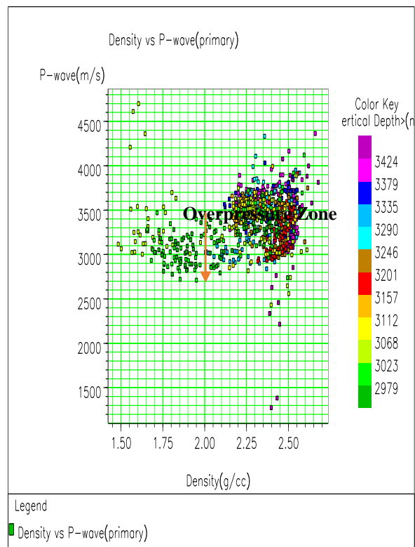
Figure 12: Velocity vs Density cross-plot for well 03. Unloading mechanism occurred from 3246m to 3335m (about 89m thick), while overpressure zones is observed from 3157m to 3201m (red colour key) and about 44m thick.
