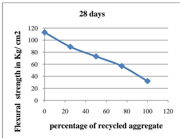
Fig. 4 shows the 28 days flexural strength of concrete with percentage of recycled aggregate concrete
