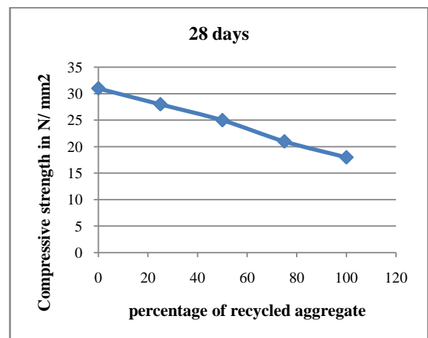
Fig. 2 shows the 28 days compressive strength of normal concrete v/s % of recycled aggregate concrete.
