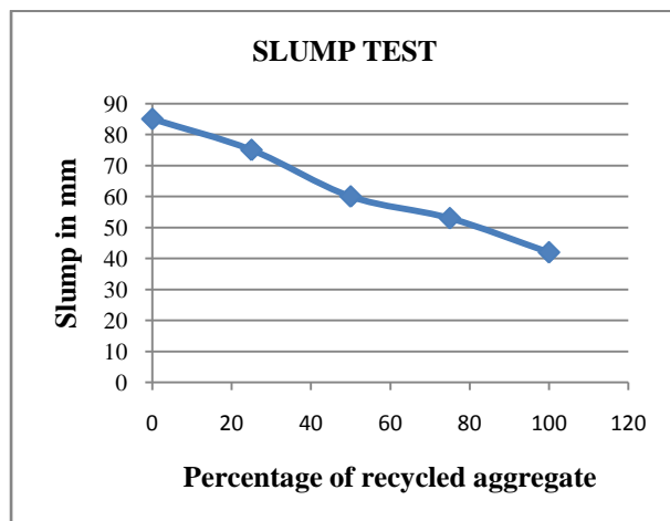
Fig. 1 shows the slump test results
