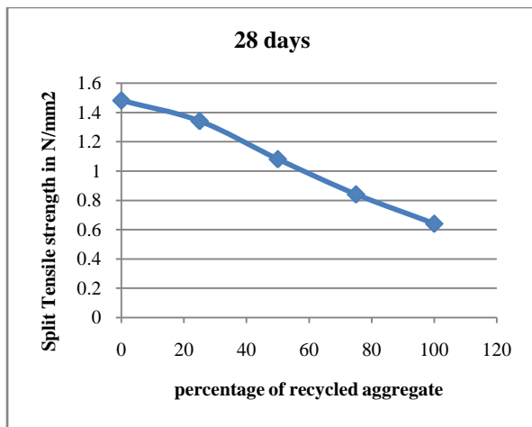
Fig. 3 shows the 28 days split tensile strength of concrete with percentage of recycled aggregate concrete
