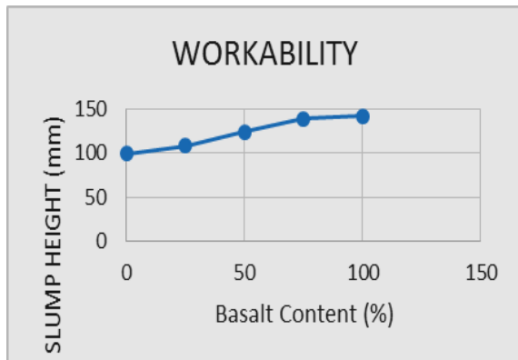
Figure.1: Graph showing results for slump test
