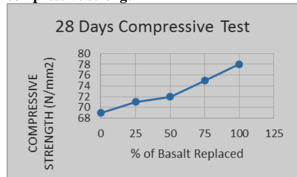
Figure2: Graph showing results for 28 days compressive strength
