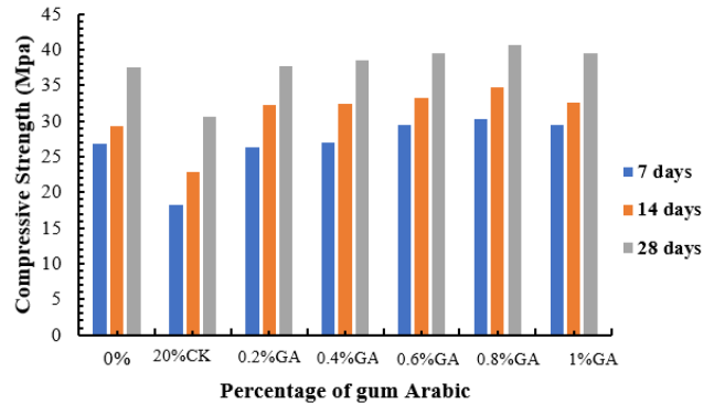
Fig. 10 Compressive strength with CK and GAB content
