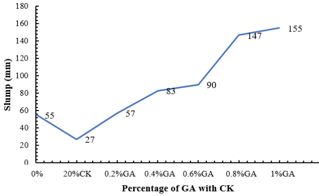
Fig. 8 Slump with CK and GAB content
