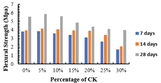
Fig. 14 Flexural strength with GAB and CK content
