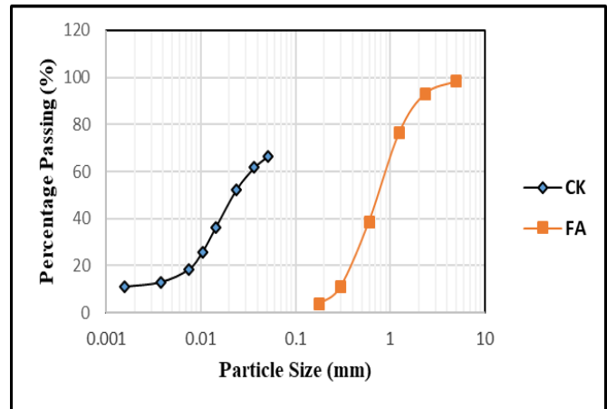
Fig. 1 Calcined Kaolin and fine aggregate distribution curve
