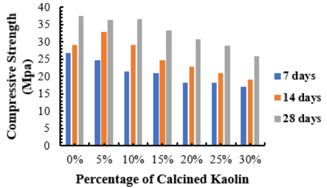
Fig. 9 Compressive strength with CK content
