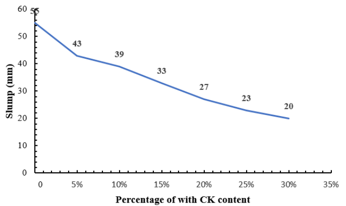
Fig. 7 Slump with CK content
