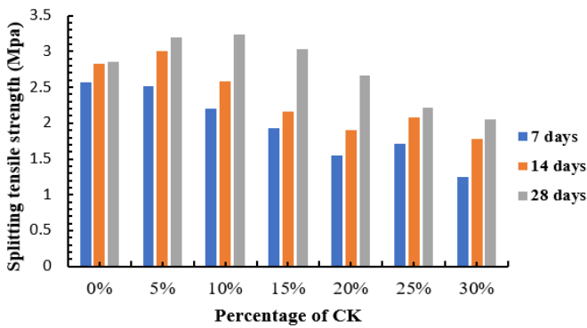
Fig.11 Splitting tensile with CK content
