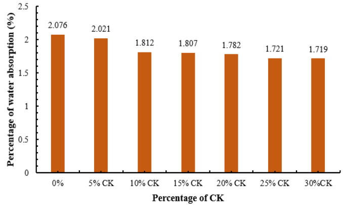
Fig. 5 Water absorption with CK content
