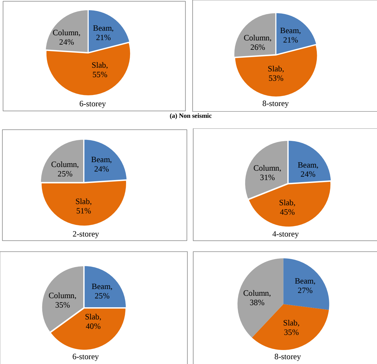
Fig. 6 Elemental contribution to embodied carbon for seismic and non-seismic designs in 2-, 4-, 6-, and 8-storey buildings
