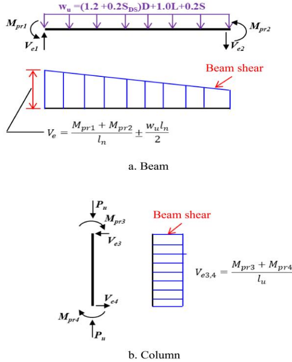
Fig. 2 Beam and column shear force design checks in seismic frames
