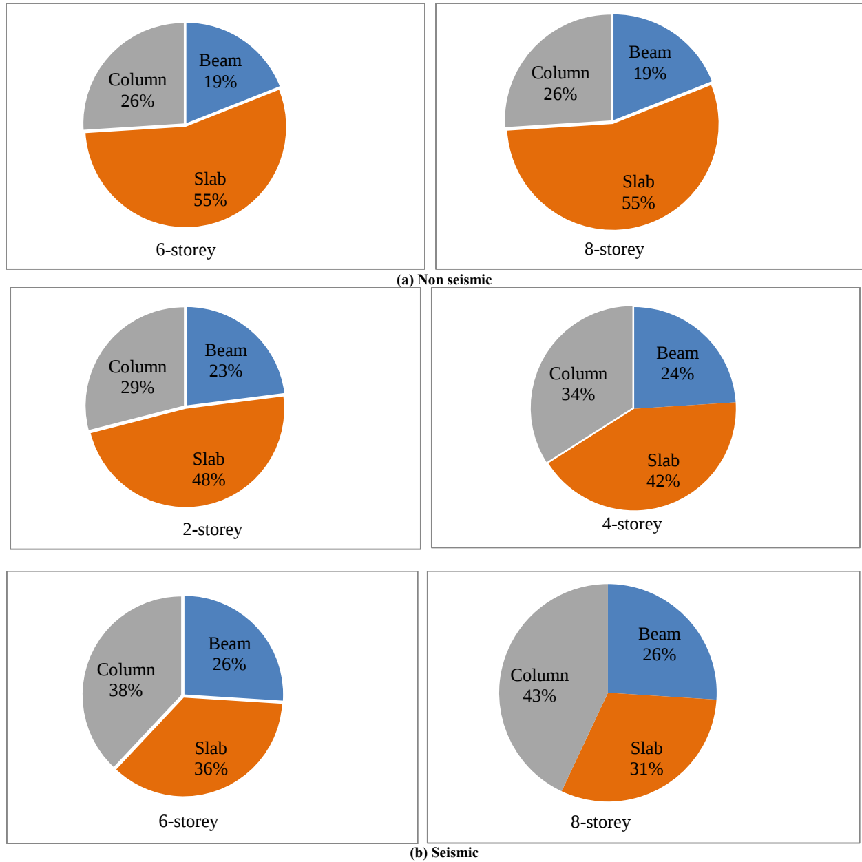
Fig. 8 Elemental contribution to cost for seismic and non-seismic designs in 2-, 4-, 6-, and 8-storey buildings
