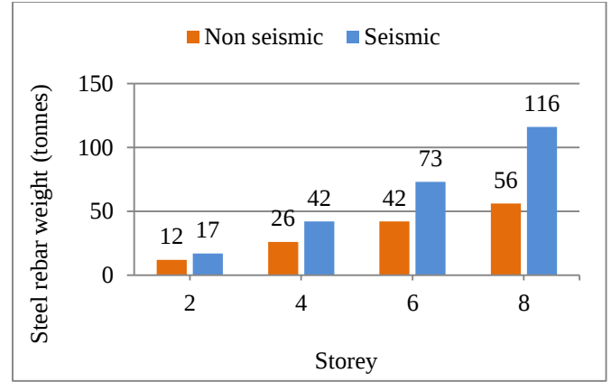
(b) Steel rebar Fig. 3 Total concrete volume and steel reinforcement weight for seismic and non-seismic designs in 2-, 4-, 6-, and 8-storey buildings
