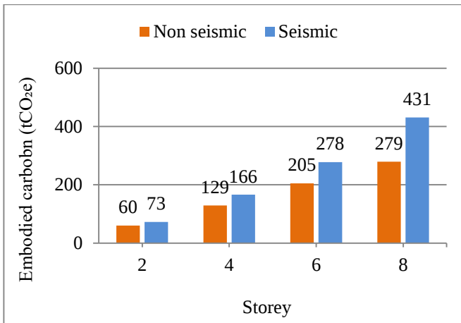
Fig. 5 Embodied carbon for seismic and non-seismic designs in 2-, 4-, 6-, and 8-storey buildings
