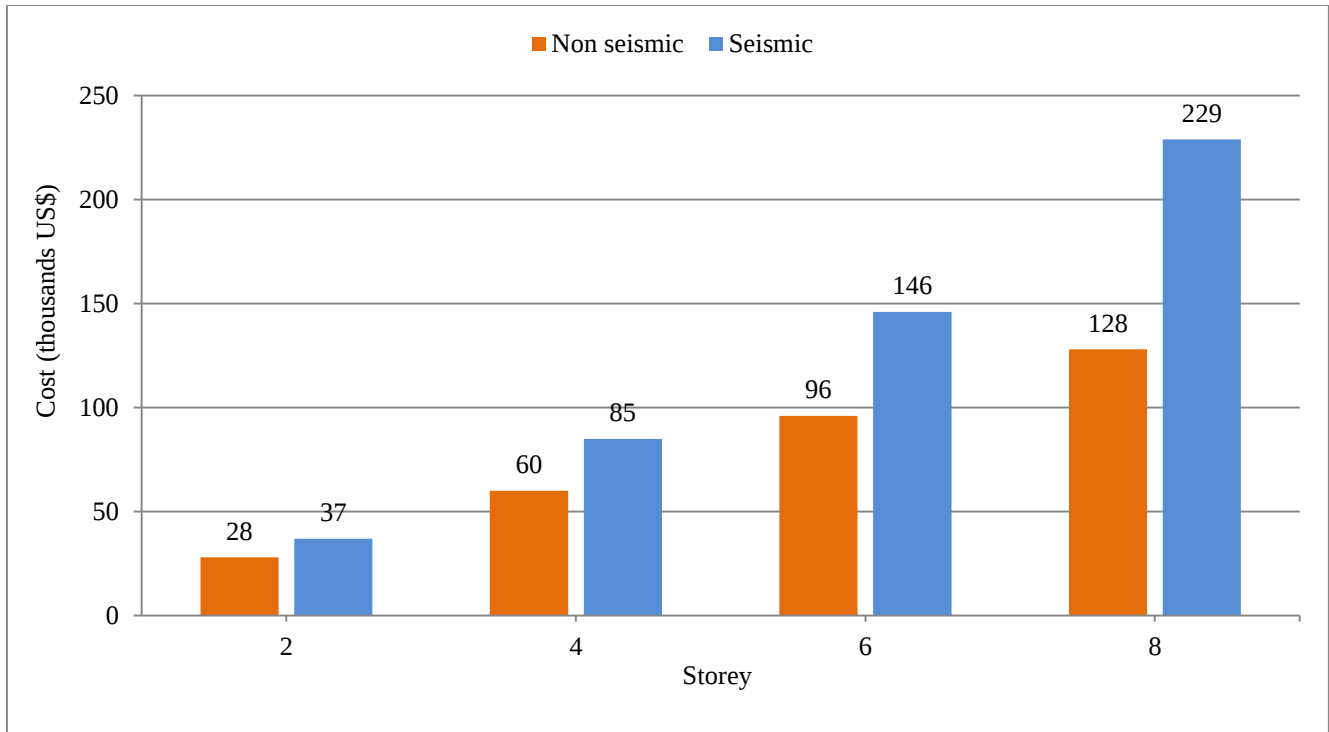
Fig. 7 Cost for seismic and non-seismic designs in 2-, 4-, 6-, and 8-storey buildings
