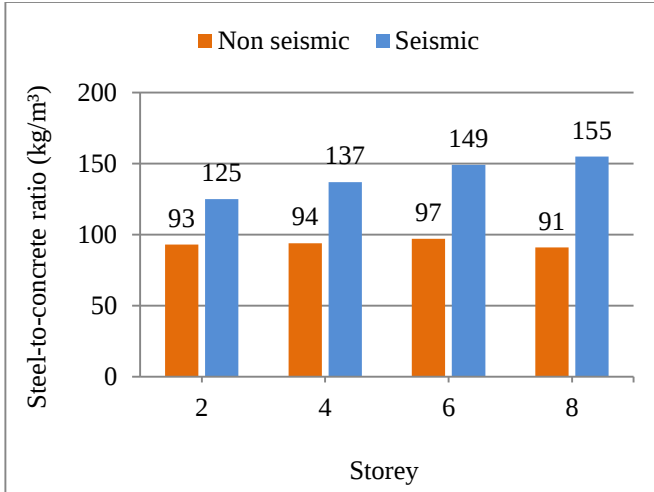
Fig. 4 Steel-to-concrete ratio for seismic and non-seismic designs in 2-, 4-, 6-, and 8-storey buildings
