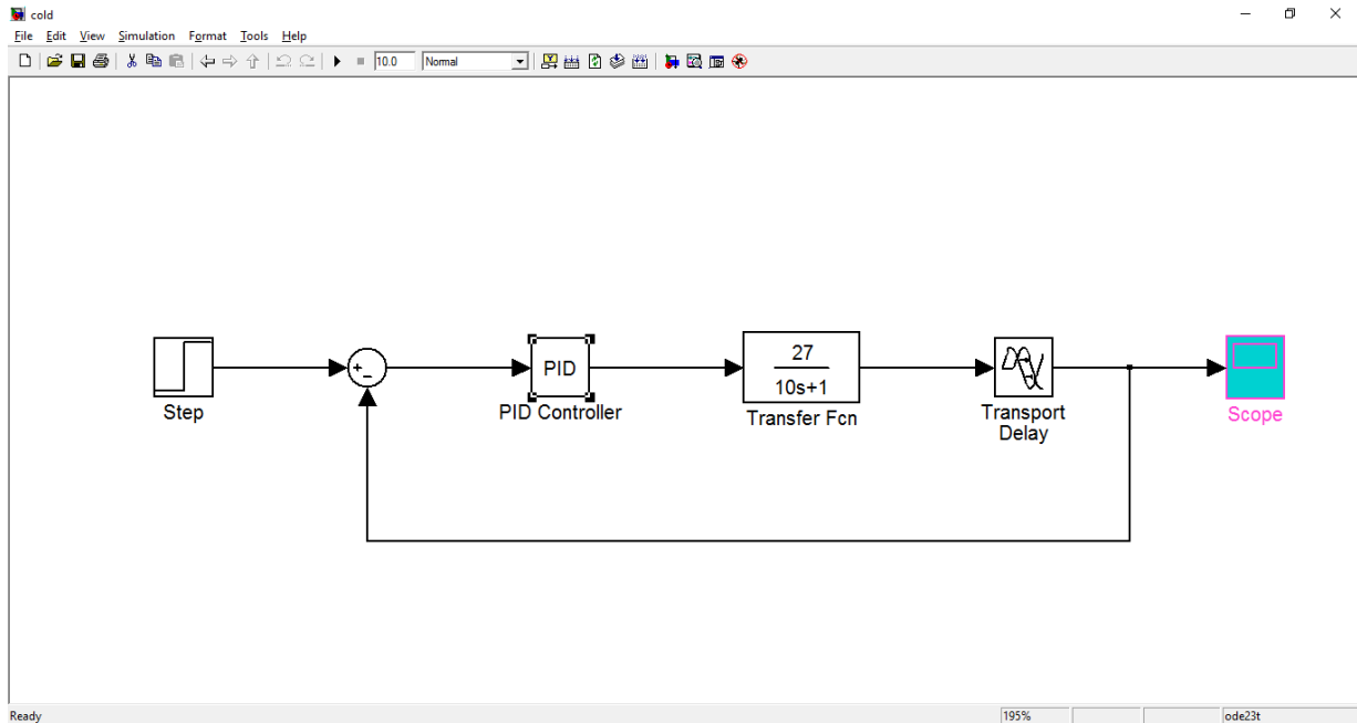
Fig 7: Block Diagram of Closed-Loop System For Cold Water Using PID Controller
