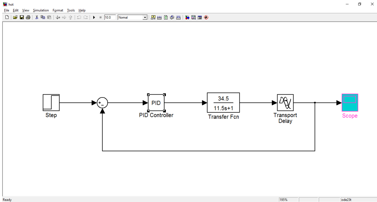
Fig 5: Block Diagram of Closed-Loop System for Hot Water Using PID Controller
