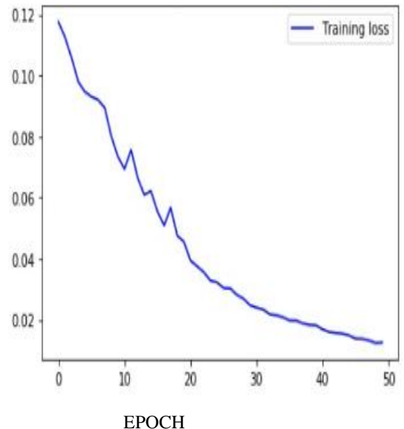
Fig 8: Loss
