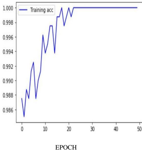
Fig 7: Accuracy
