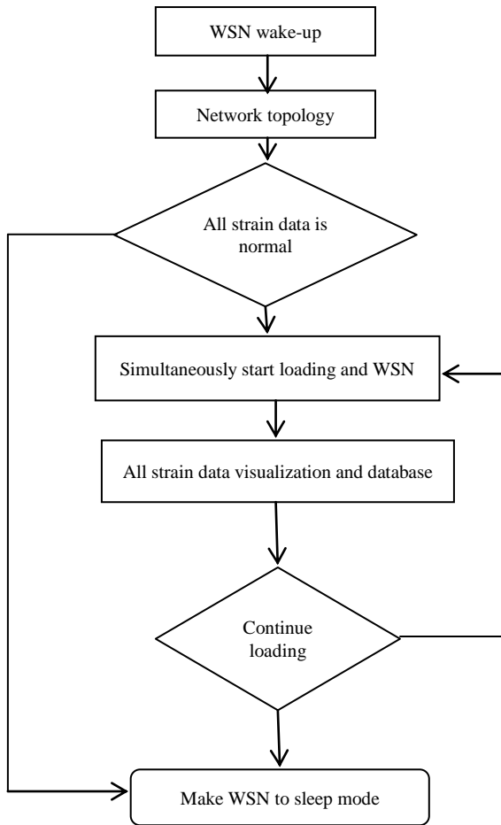
Fig .2 Flow Diagram of FNR
