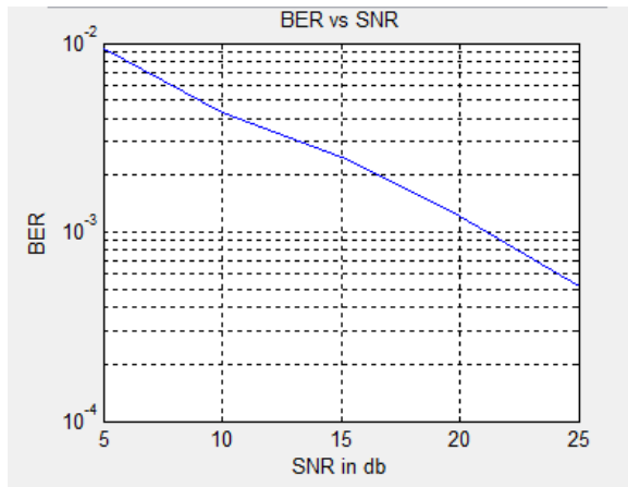
Fig 5. SNR v/s BER for MIMO-OFDM using STBC
