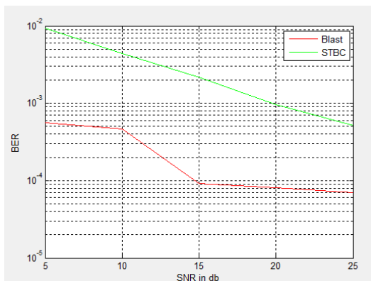
Fig 6. Comparison of SNR vs BER for Both MIMO-OFDM using V-Blast & MIMO-OFDM using STBC
