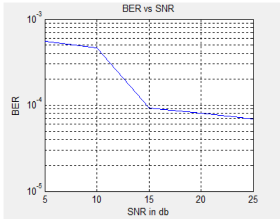
Fig 4. SNR v/s BER For MIMO-OFDM using V-BLAST
