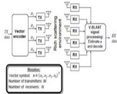
Fig 1. V-Blast Architecture
