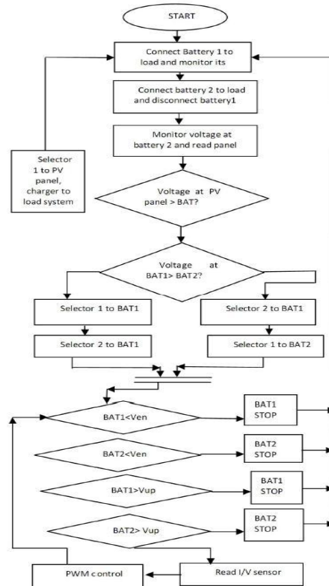
Fig. 4. Charging and Discharging Algorithm
