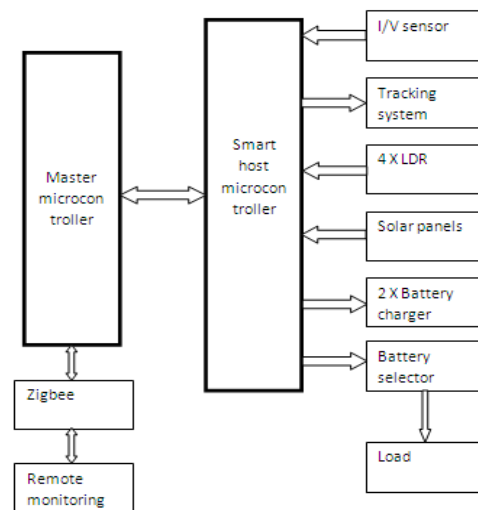
Fig.2. Block Diagram of Hardware Architecture of System
