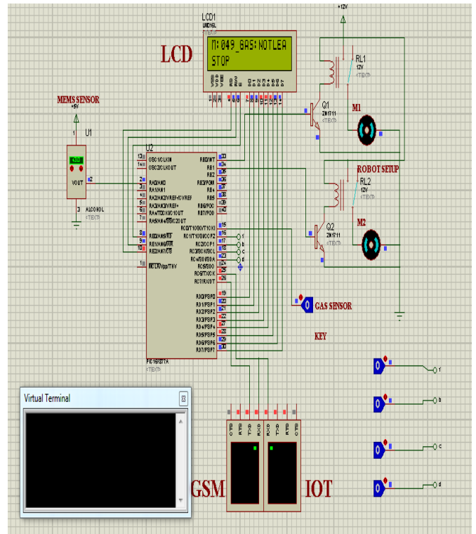
FIG: 3 location tracker
