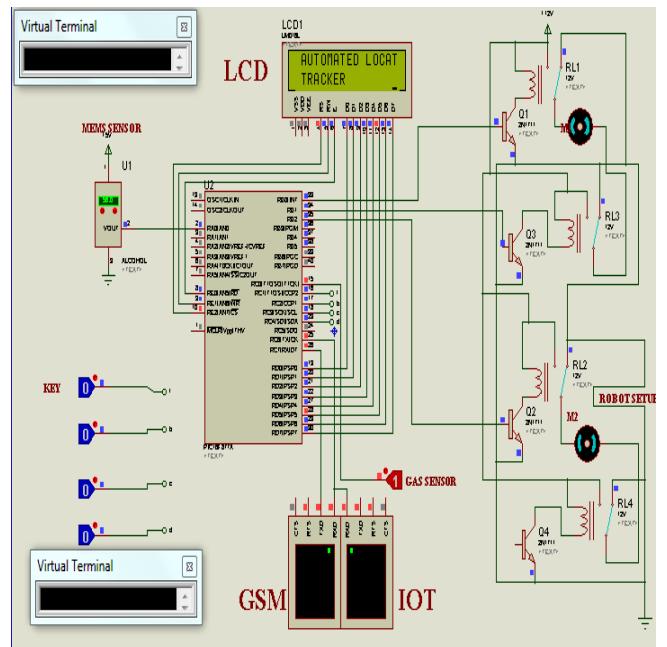
FIG: 4 simulation output under normal condition
