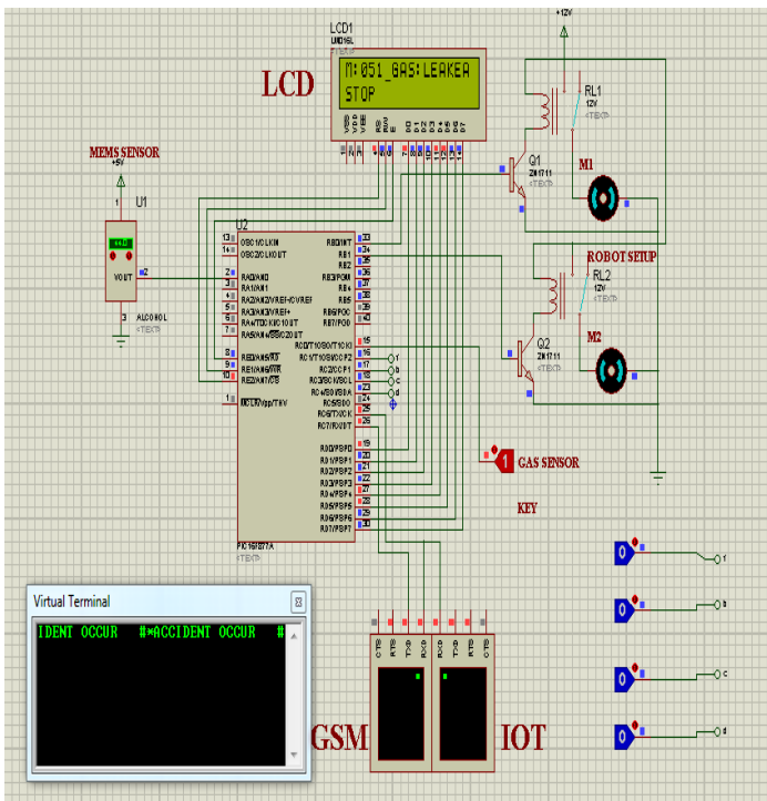
FIG :6 simulation output during Gas Leakage
