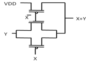
Fig 5: TG OR logic
