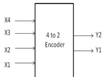
Fig :1 General 4-2 encoder block
