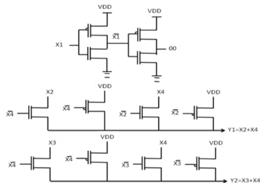
Fig 7: 4-2 Encoder using DPL
