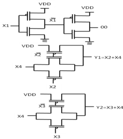
Fig 9: 4-2 Encoder using TG logic
