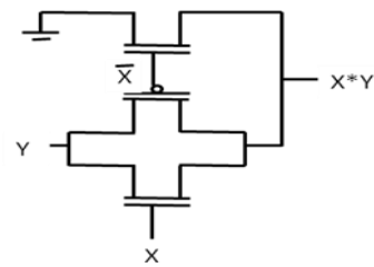
Fig 6: TG AND logic
