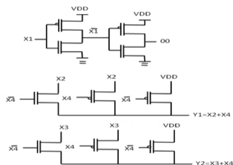
Fig 8: 4-2 Encoder using DVL
