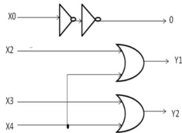
Fig 2: 20-Transistors 4-2 line encoders
