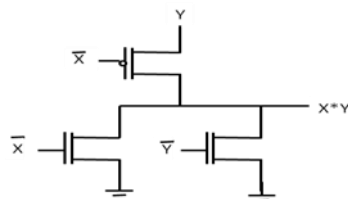
Fig 4 :DVL AND logic
