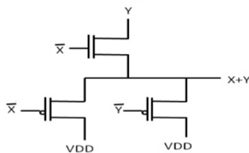
Fig 3:DVL OR logic
