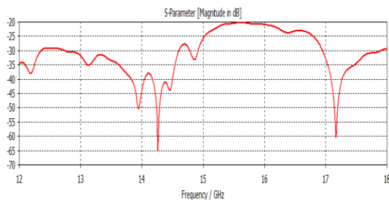
Fig. 2, Simulated Return Loss Characteristics of Turin Conical Horn Antenna without Corrugation
