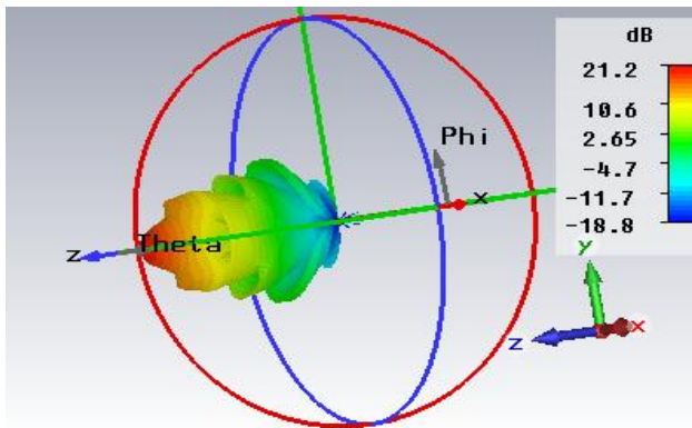
Fig. 10, Simulated 3-D Radiation Pattern of the Smooth Walled Turin
