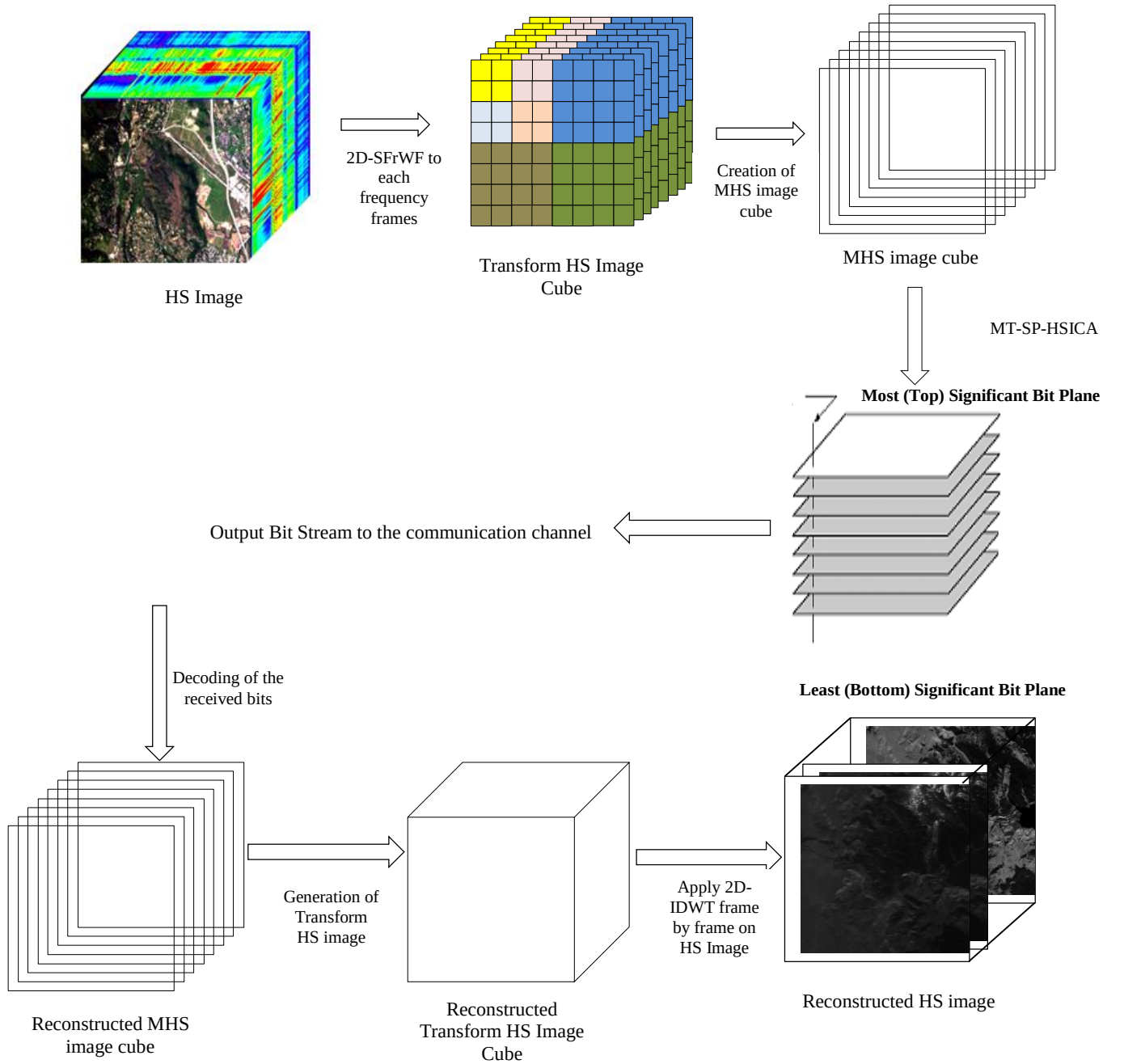
Fig. 1 Processing pipeline for the proposed compression algorithm
