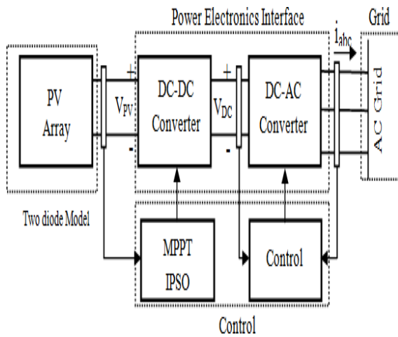
Fig 1: Block Diagram of Solar PV Grid System
