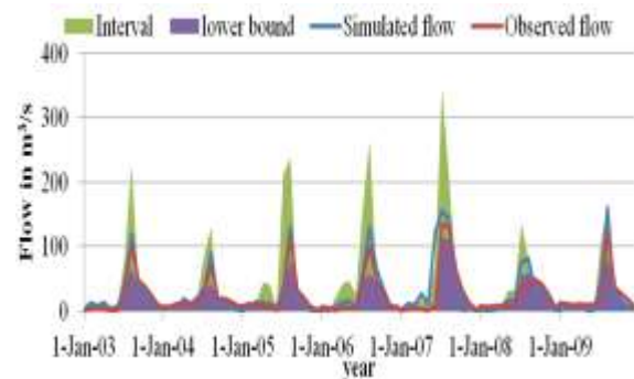
Fig.12. Uncertainty analysis in HBV light model
