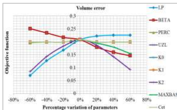
Fig.6. Sensitivity analysis by considering volume error
