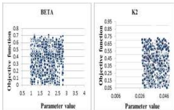
Fig. 11. Dotty plot for model parameters
