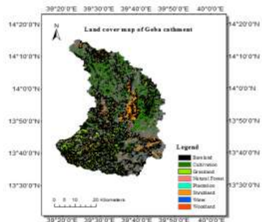
Fig.3. Landuse land cove map of the study area
