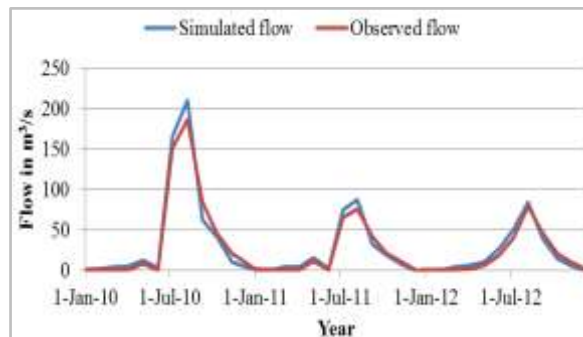
Fig.9. Observed and simulated hydrographs during validation period.
