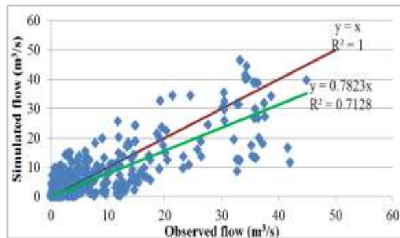
Figure8. Scatter plot during calibration period in the Geba cathment
