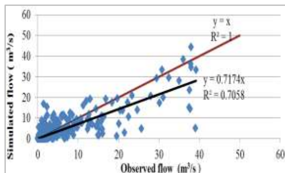
Fig.10. Scatter plot during validation period in the Geba cathment.
