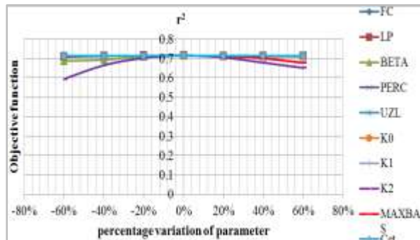
Fig.4. Sensitivity analysis by considering R^2
