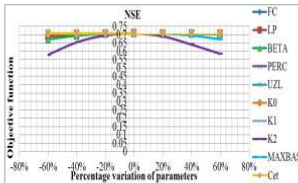
Fig.5. Sensitivity analysis by considering NSE
