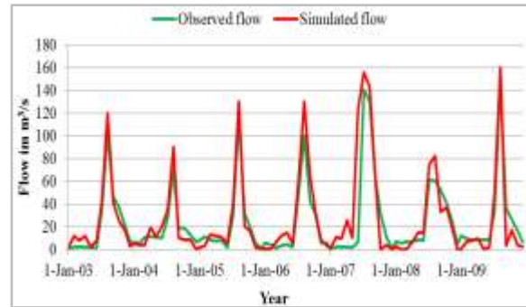
Fig.7. Observed and simulated flow hydrographs during calibration period
