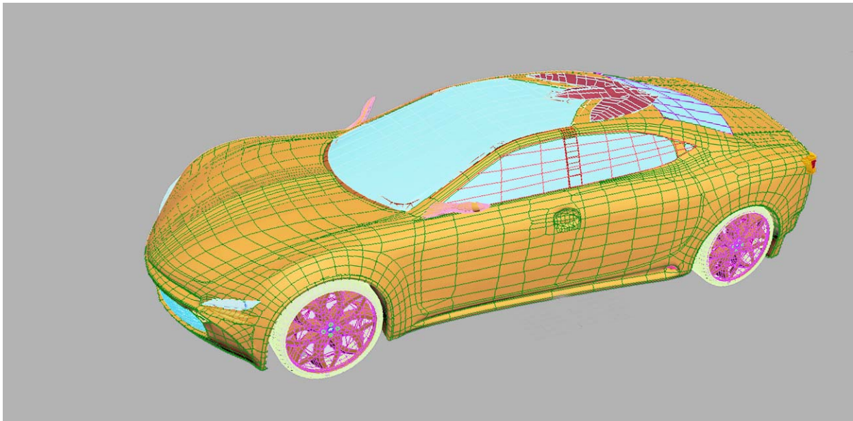
Fig. 4. Three-dimensional smoothed surface of body
