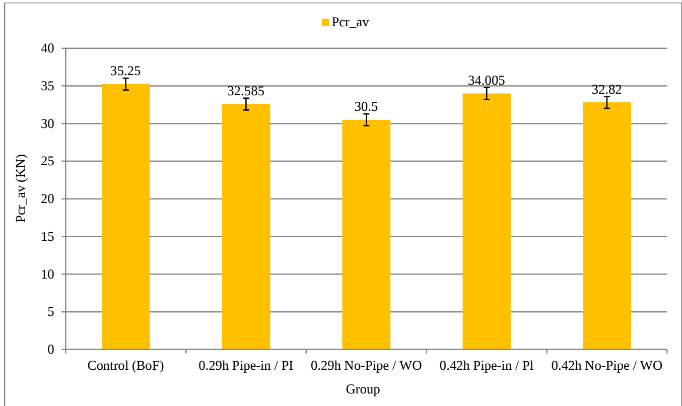
Fig. 6 Mean first-crack load PCR for the five flexural beam groups
