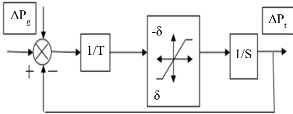
Fig. 3 Non-linear turbine model with GRC
