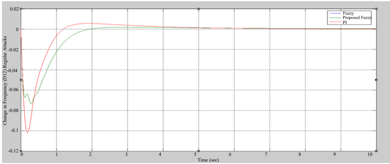
Fig. 10 Variations in frequency of area two ( \Delta f_2 ) with regular attacks
