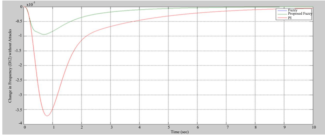
Fig. 7 Variations in frequency of area two ( \Delta f2 ) without attacks
