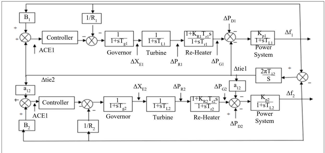
Fig. 2 Basic Block Diagram of the two area system
