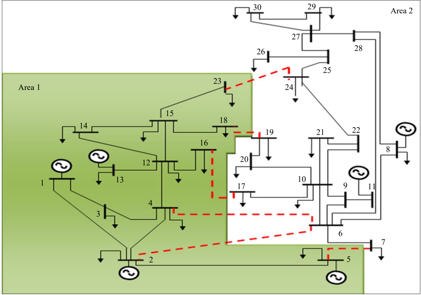
Fig. 1 IEEE 30 bus two area system
