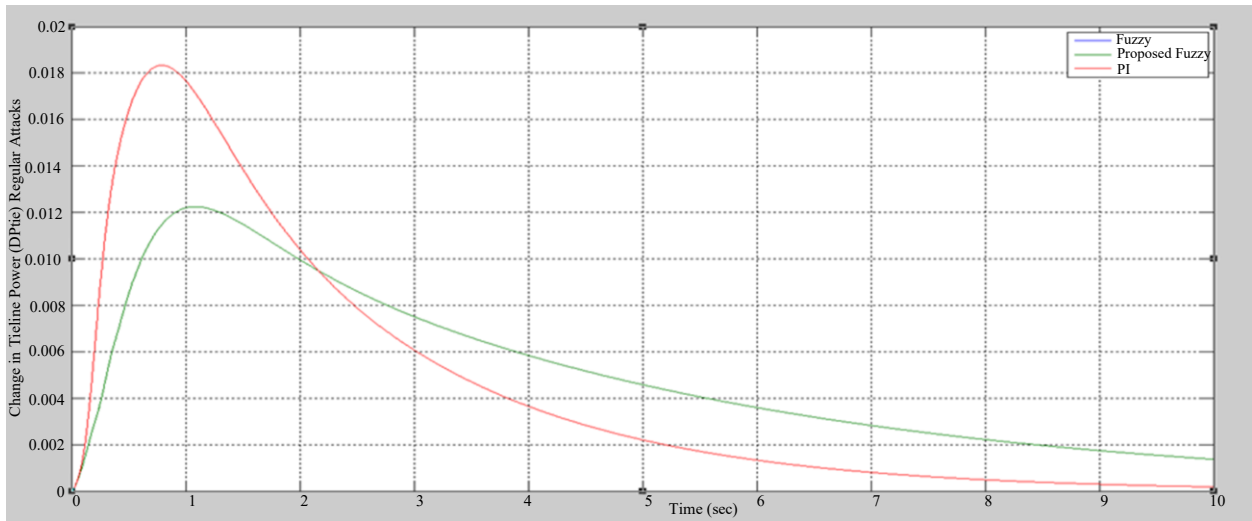
Fig. 11 Variations in tie line power ( \Delta P_{tie} ) with regular attacks
