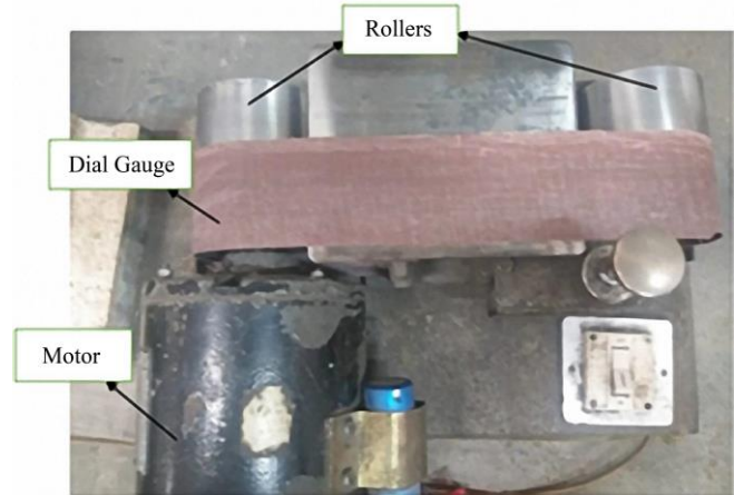
Fig. 6 Belt grinder
