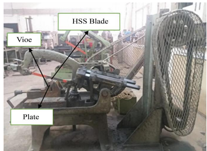
Fig. 1 Power hacksaw
