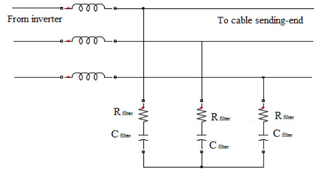
Fig.4 RLC filter at the inverter output
