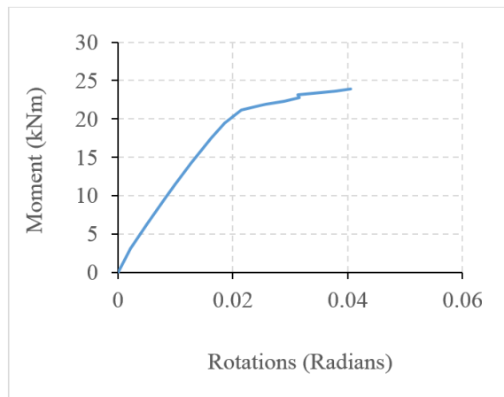
Fig.6 Moment vs Rotation curve
