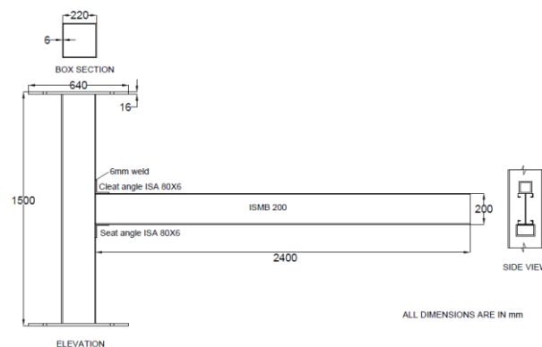
Fig.1 Sketch of beam-to-column connection
