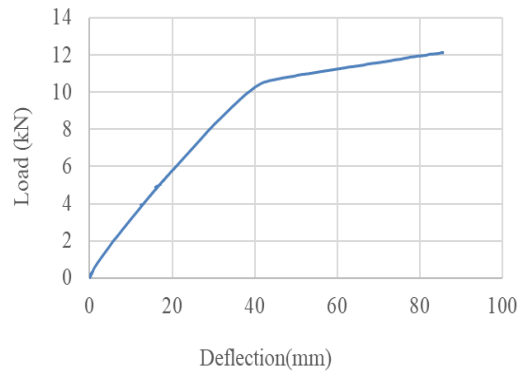
Fig 5. Load vs Deflection behaviour
