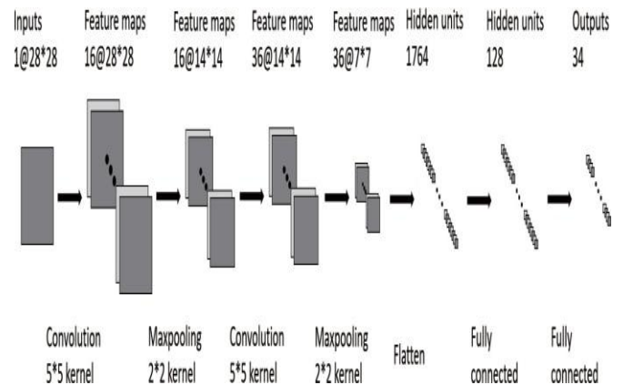
Fig.7.the proposed LPRCNN for license plate character recognition
