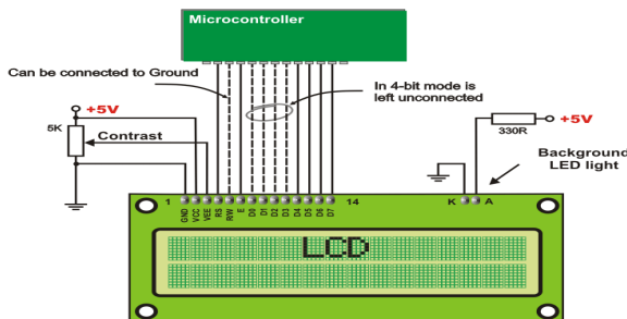
Figure 4. Interfacing LCD to Microcontroller
