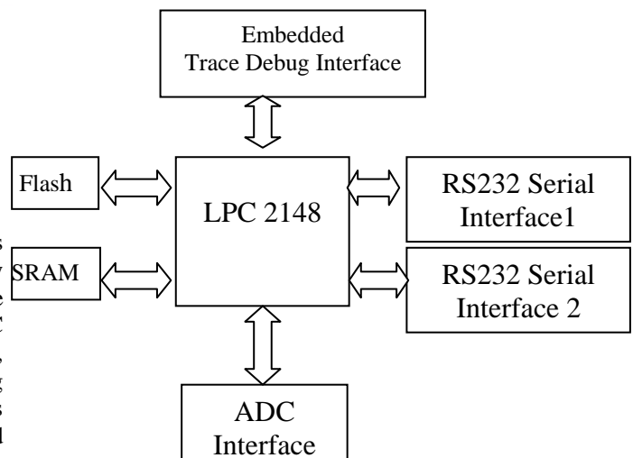
Figure 2. The Hardware Structure of Processing Terminal.
