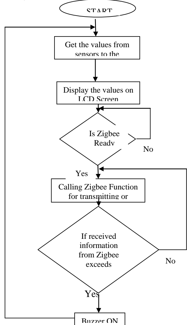
Figure 8.Flow chart for the Under Ground Section.
