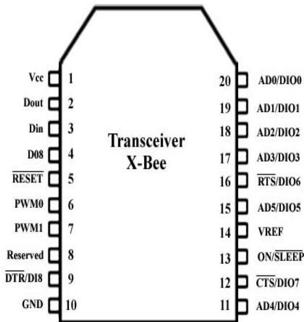
Figure 6.Pin Diagram of Zigbee Transceiver.
