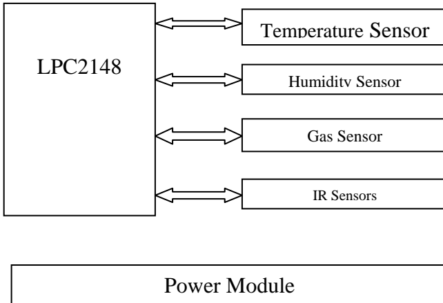
Figure 3. Hardware Structure of Sensor node.
