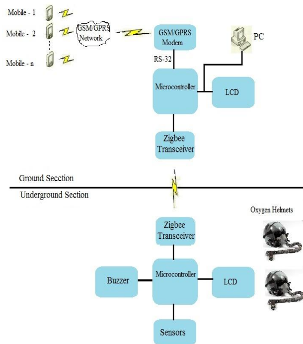
Figure 1. Block Diagram of Designed System
