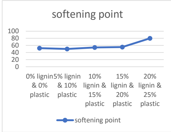
Fig 5.2. Percentage of replacement vs Softening point(°c)
