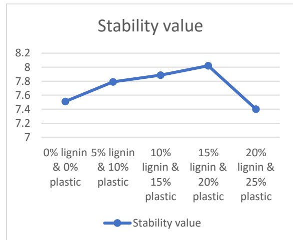
Fig 5.5. Percentage of replacement vs Stability value
