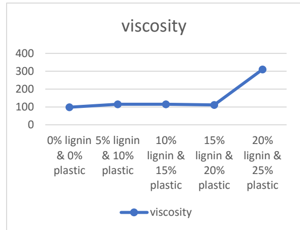
Fig 5.4. Percentage of replacement vs Viscosity(secs)
