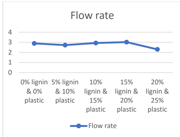
Fig 5.6. Percentage of replacement vs Flow rate
