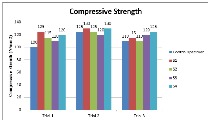
Fig: 1 COMPRESSIVE STRENGTH TEST
