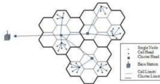
Fig-5: Cell-LEACH Protocol [19]
