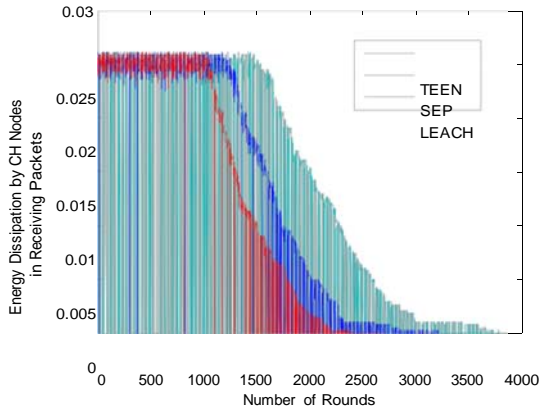
Fig-8: Energy dissipated by CH Nodes Vs Number of Rounds
