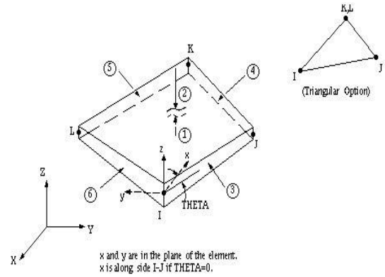
Fig.6 Element shell 41
