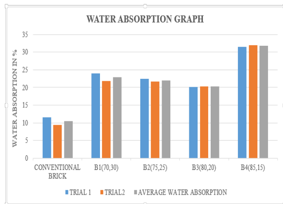
Figure 4.3 Graph of Water Absorption test
