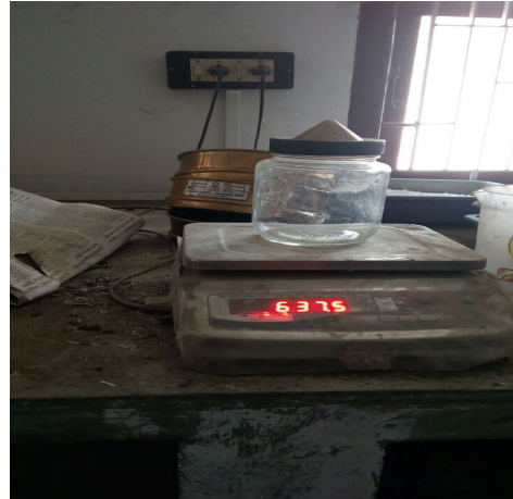
Figure:3.1.specific gravity test
