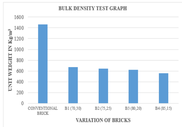
Figure:4.1. graph for bulk density test results
