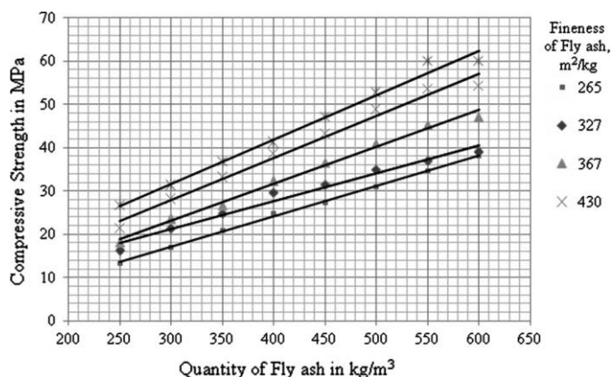
Fig. 3 Effect of quantity of fly ash on compressive strength for different fineness at solution-to-fly ash ratio
