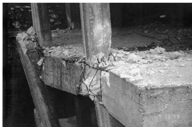
Figure 2 Typical View of Beam-Column Joint Failure (Reference: www.researchgate.net )
