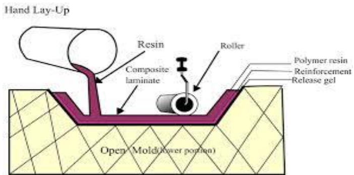
Fig 4.1 Hand Lay-up Method
