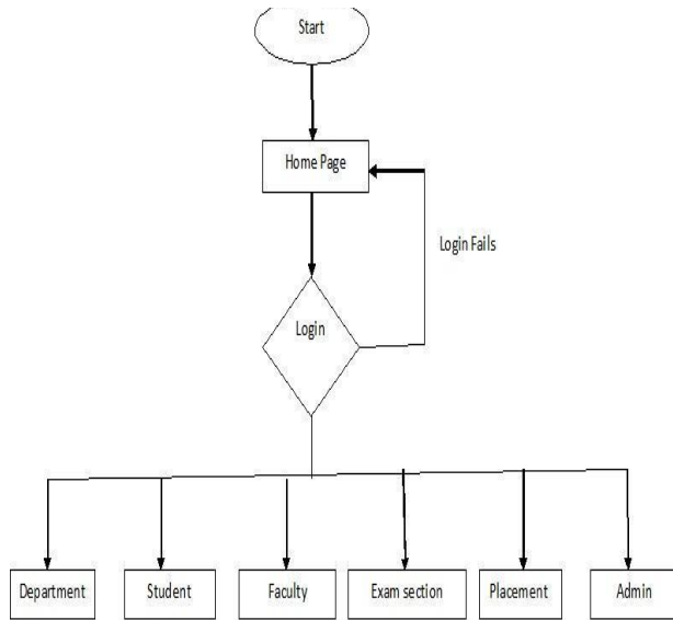
Fig1:Login process
