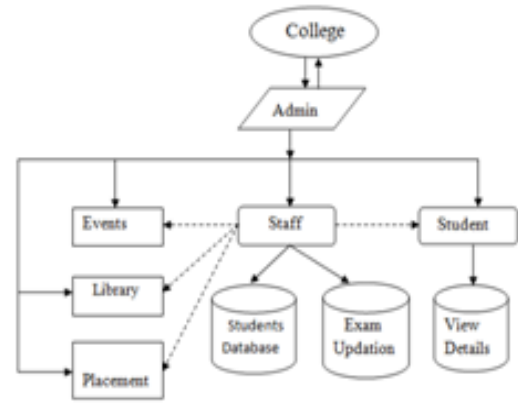
Fig2:System Architecture
