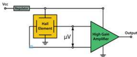
Fig.2-Hall effect sensor
