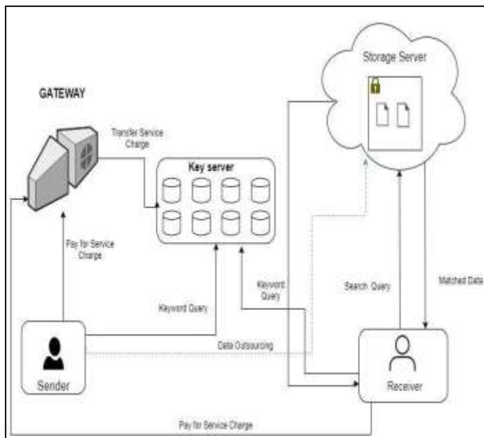
Figure 3: Proposed Architecture.
